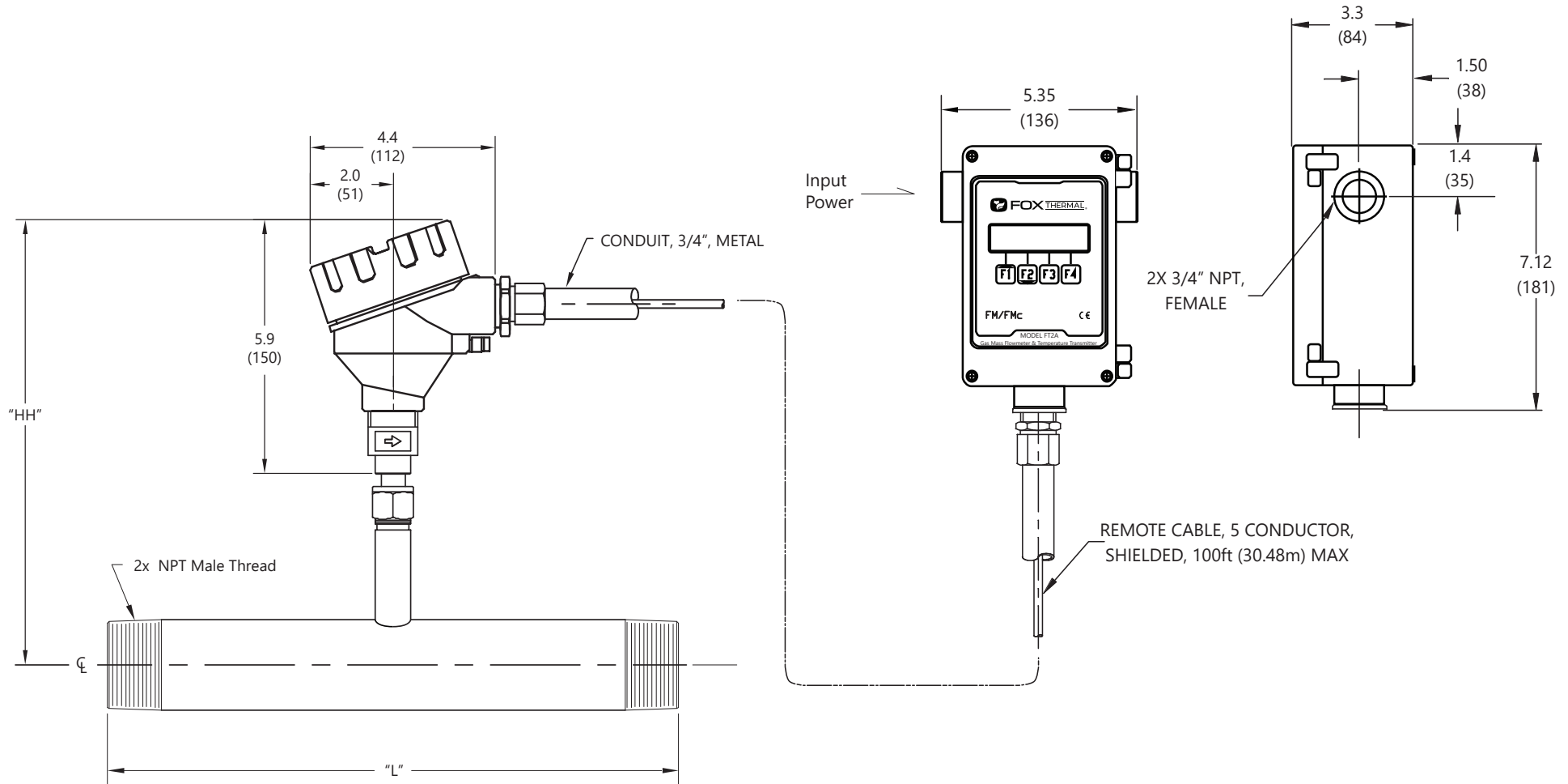
Model FT2A Dimensions
