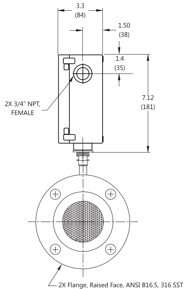
Model FT2A Dimensions
