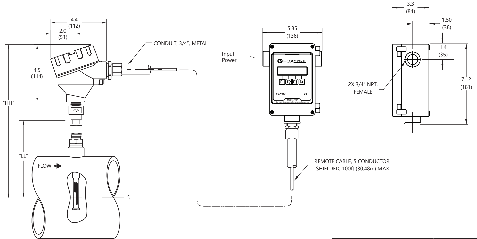
Model FT2A Dimensions
