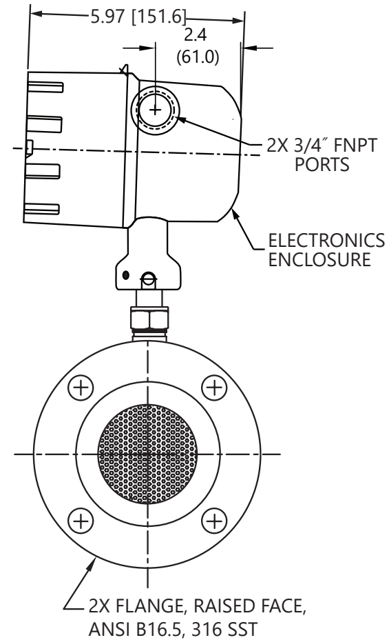
Model FT4A Dimensions
