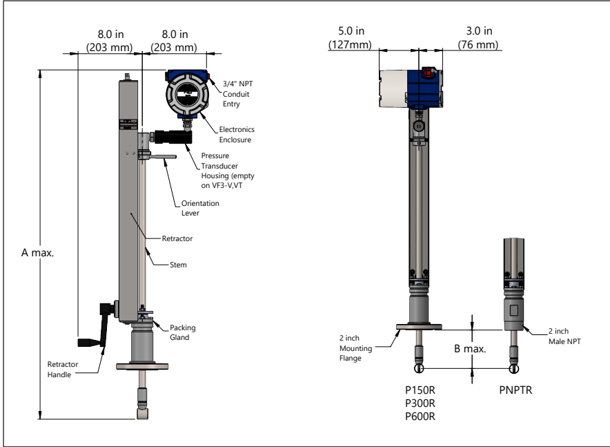
VF3 Packing Gland, Retractor
